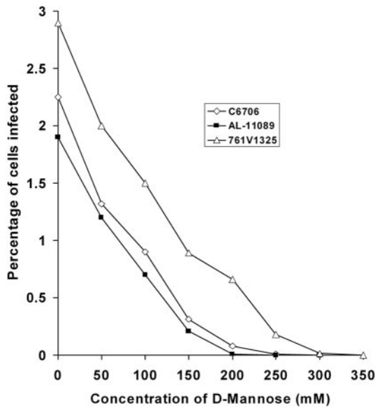
FIG. 2. Effect of D-mannose on the susceptibility of V. cholerae strains to KSF1-KmΦ. The identity (and serotype) of strains tested are C6706 (O1, El Tor), AL-11089 (O139), and 761V1325 (non-O1/non-O139).
